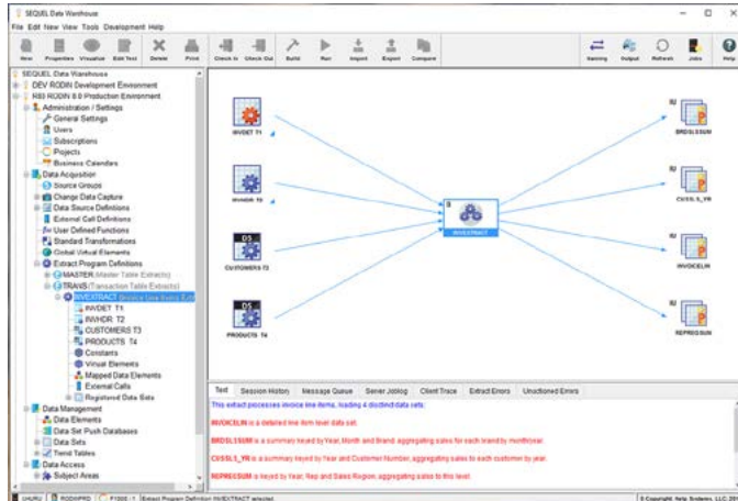
Sequel Data Warehouse ETL overview
